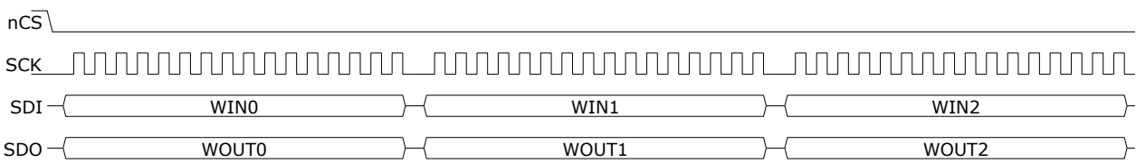
Figure 14 Arrangement of SPI words
