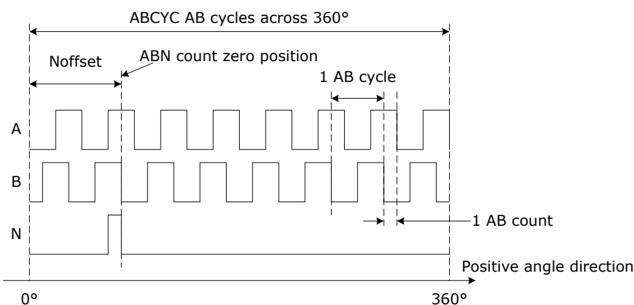
Figure 24 ABN signals as a function of position
