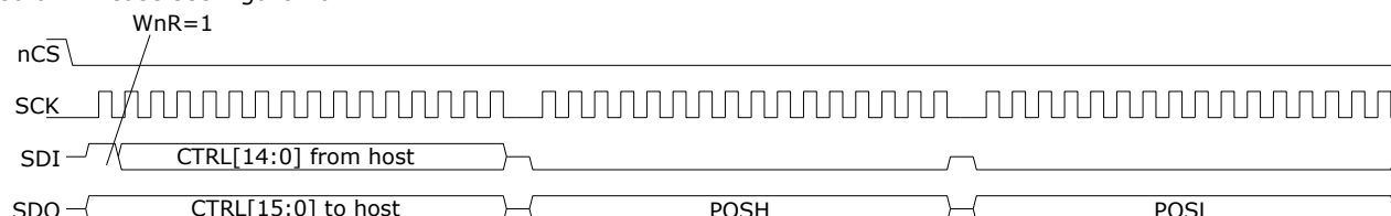
Figure 16 Register write-read operation
