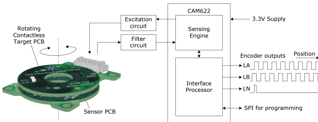
Figure 3 CAM622 function overview
