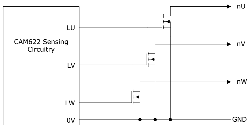
Figure 39 Generating open drain U, V, W signals using external MOSFETs
