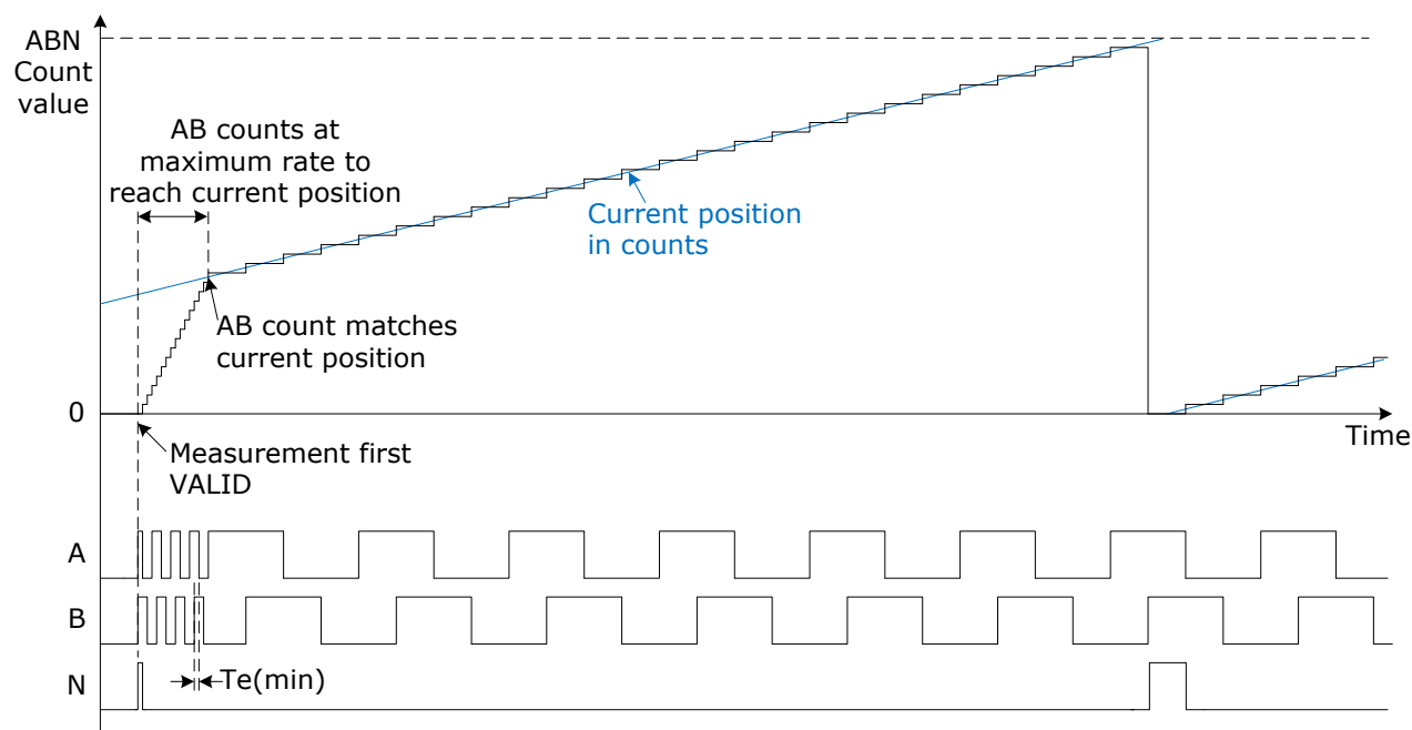
Figure 28 ABN behaviour following first VALID with NSTART=1
