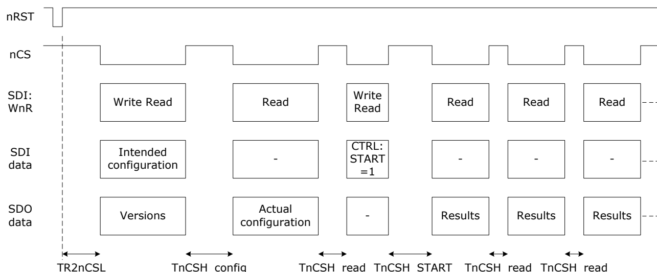
Figure 18 SPI transactions for taking repeated measurements
