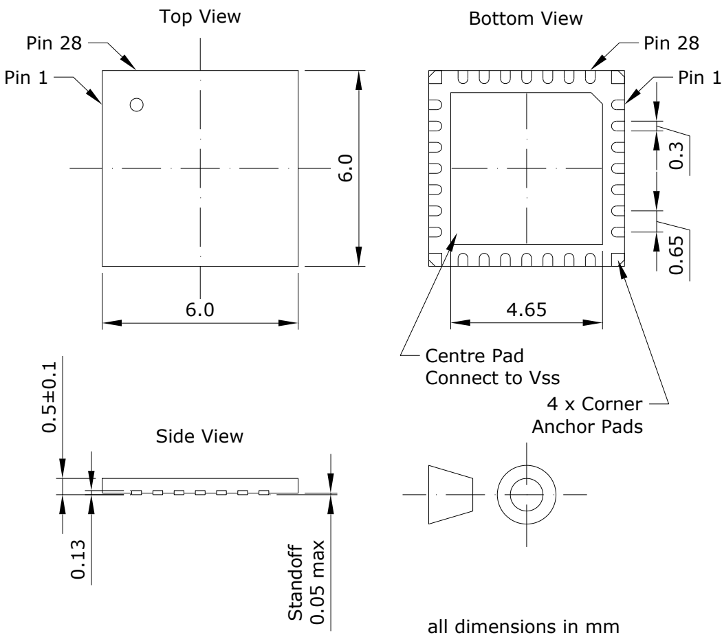
Figure 49 CAM622UE plastic quad-flat no-lead 28-pin (UQFN: U suffix)
