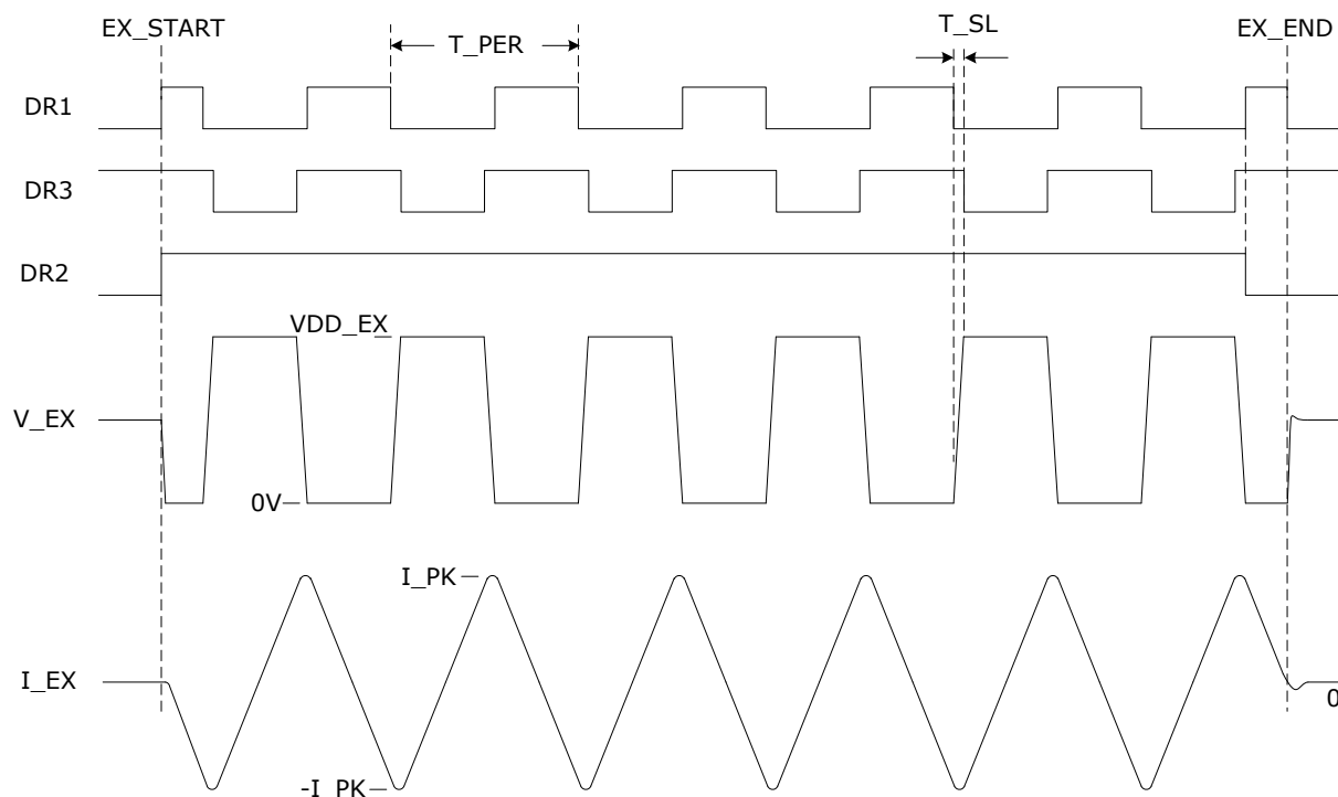
Figure 7 Excitation waveforms
